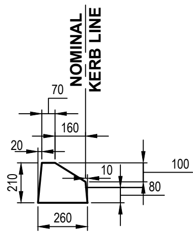
RMS KERB TYPE 'SF' SCALE 1:20 REF: RMS STD DRG R0300-01
