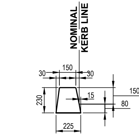
RMS KERB TYPE 'SM' SCALE 1:20 REF: RMS STD DRG R0300-01
