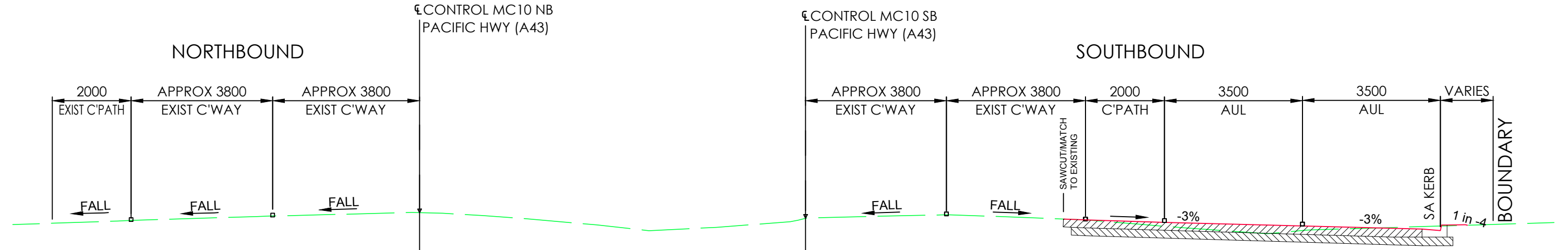
PACIFIC HWY (A43) >CH1000 TYPICAL CROSS SECTION SCALE 1:100
