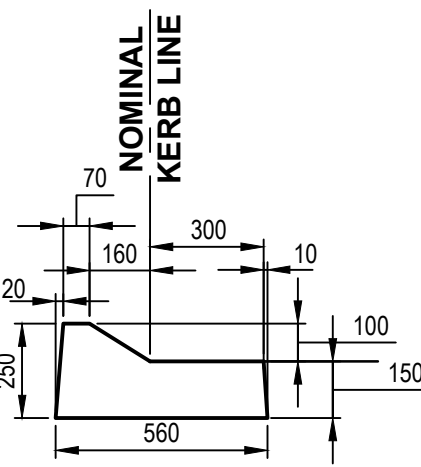
RMS KERB TYPE 'SE' SCALE 1:20 REF: RMS STD DRG R0300-01
