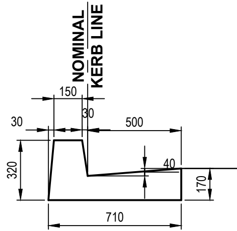
RMS KERB TYPE 'SA' SCALE 1:20 REF: RMS STD DRG R0300-01
