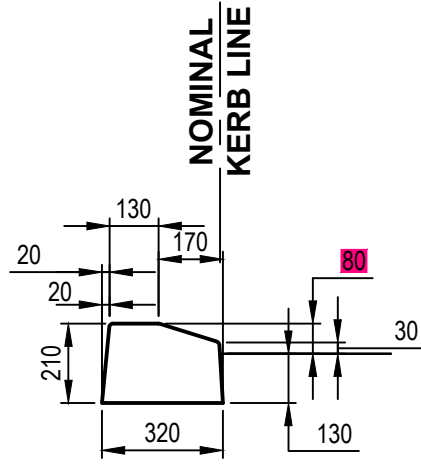
KERB TYPE 'SFA' SCALE 1:20 SPECIAL 'SF' TYPE FOR RNB ANNULUS ENCROACHMENT TYPE A
