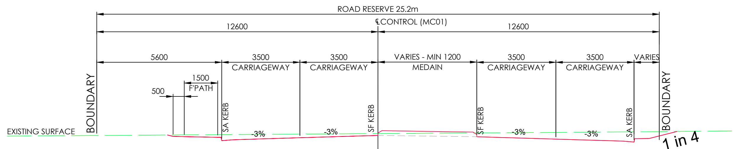
ROAD 01 (MC01) TYPICAL CROSS SECTION SCALE 1:100
