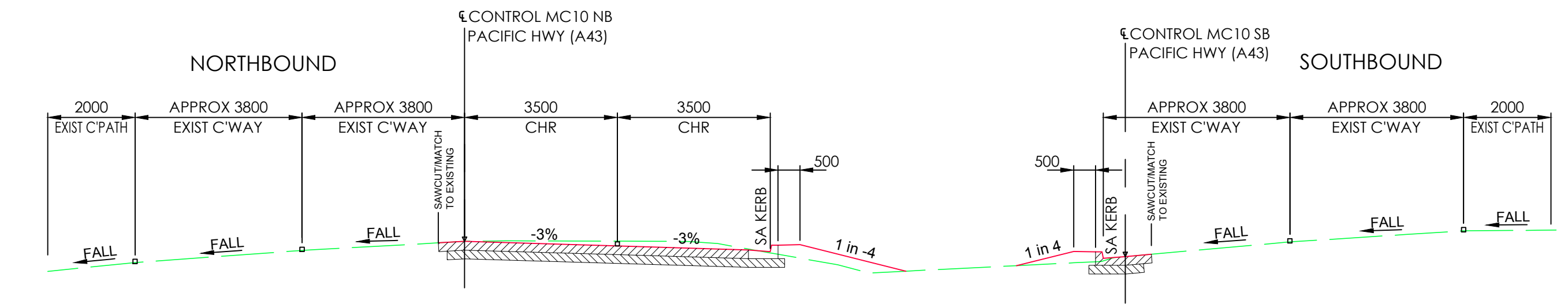
PACIFIC HWY (A43) <CH1000 TYPICAL CROSS SECTION SCALE 1:100
