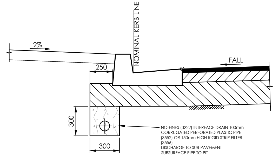
TYPICAL PAVEMENT EDGE DETAIL SCALE 1:20
