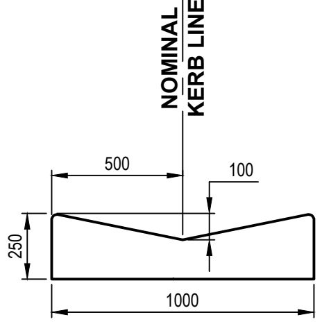
RMS KERB TYPE 'SO' SCALE 1:20 REF: RMS STD DRG R0300-01
